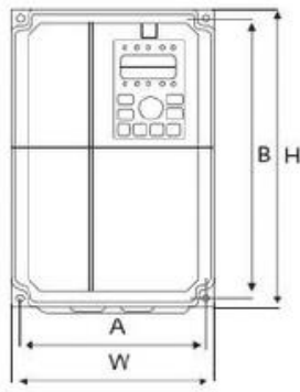
Figure 2-3 Dimensions below 22kw plastic model
