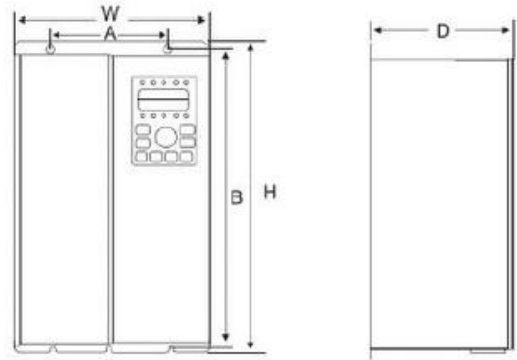
Figure 2-4 Boundary Dimensions of 30-500KW
